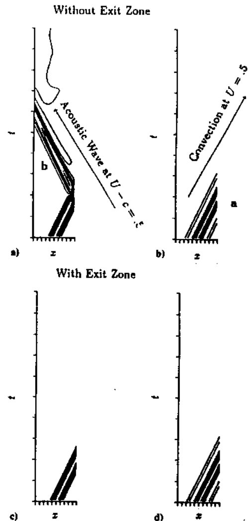
Fig. 8 Propagation of a vortex in uniform flow, M = 0.5 ; comparison of computations with and without exit zones on x-t diagrams. Shown are contours of a) pressure without exit zone, b) vorticity without exit zone, c) pressure with exit zone, and d) vorticity with exit zone. Boldface letters refer to specific events mentioned in the text. All computations with BCI2 and BCO3. Contours: pressure—min = 71.368, max = 71.459, increment = 0.007; vorticity—min = -2.0, max = 0.8, increment = 0.4.
