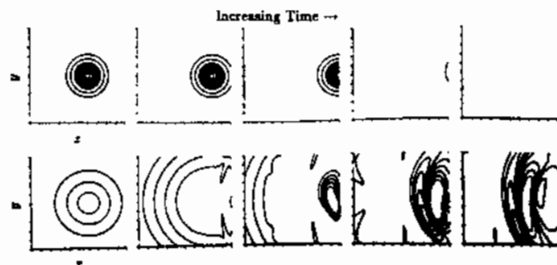
Fig. 6 Acoustic wave reflection by vortex propagating through outflow boundary. In the top row, the isocontours of vorticity are \min = -0.1 , \max = 0.8 , and increment = 0.05 . In the bottom row, the isocontours of the dilatation are \min = -0.01 , \max = 0.01 , and increment = 0.001 .
