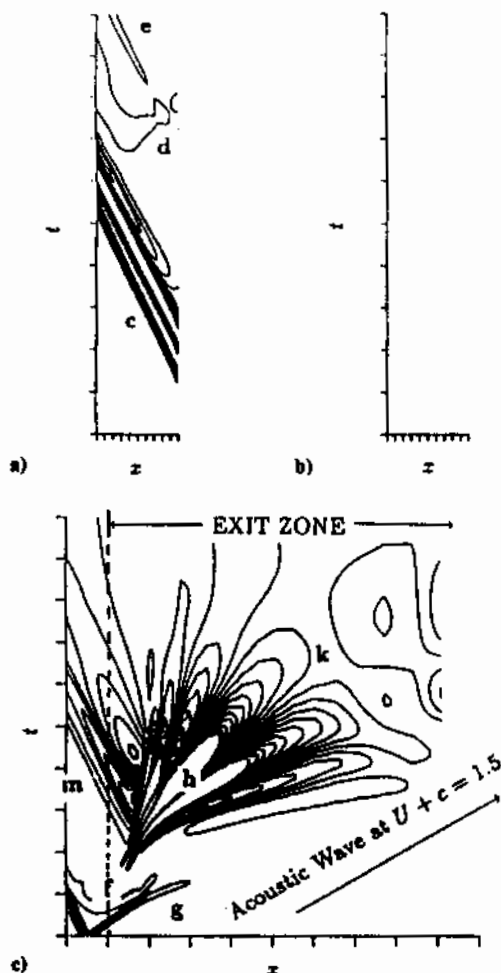
Fig. 9 Propagation of a vortex in uniform flow, M = 0.5 ; comparison of computations with and without exit zones on x-t diagrams. Shown are contours of a) dilatation without exit zone, b) dilatation with exit zone (levels: min = -0.02 , max = 0.02 , increment = 0.002 ), and c) contours of dilatation including exit zone (levels: min = -0.0002 , max = 0.0002 , increment = 0.00002 ). Boldface letters refer to specific events mentioned in the text.
