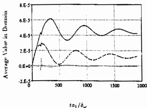
Fig. 10 Change in average u , v , \rho , and p in computational domain as a function of time: —, u ; ·····, v ; - - -, \rho ; - · - ·, p (lines for \rho and p fall directly on top of one another). Mixing layer with streamwise length of x = 60\delta_\omega . The small bump in the curves near ta_1/\delta_\omega = 160 is due to the passage of the startup vortex through the outflow boundary.
