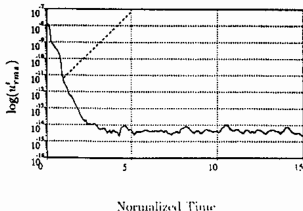
Fig. 5 Comparison of boundary conditions, decay of streamwise velocity fluctuations in uniformly sheared flow after acoustic source is turned off. Time is normalized by the average time for a particle to traverse the computational domain: —, BCI2, BCO2, and \epsilon = 0.05 ; ---, BCI2, BCO2, and \epsilon = 0 .
