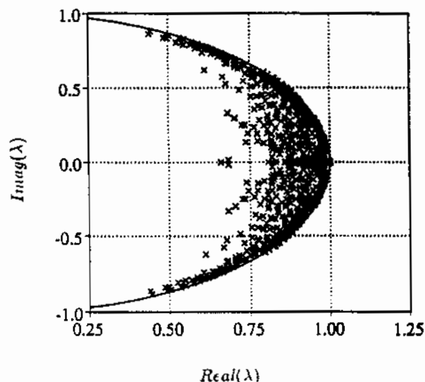
Fig. 1 Location of the eigenvalues of M in the complex plane; the solid line is the unit circle.
