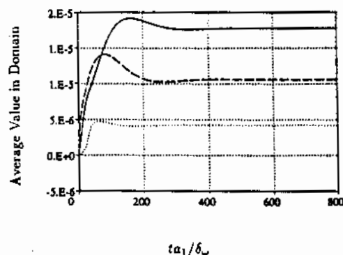
Fig. 11 Change in average u , v , \rho , and p in computational domain as a function of time: —, u ; ·····, v ; - - -, \rho ; - · - ·, p (lines for \rho and p fall directly on top of one another). Mixing layer with streamwise length of x = 10\delta_\omega .
